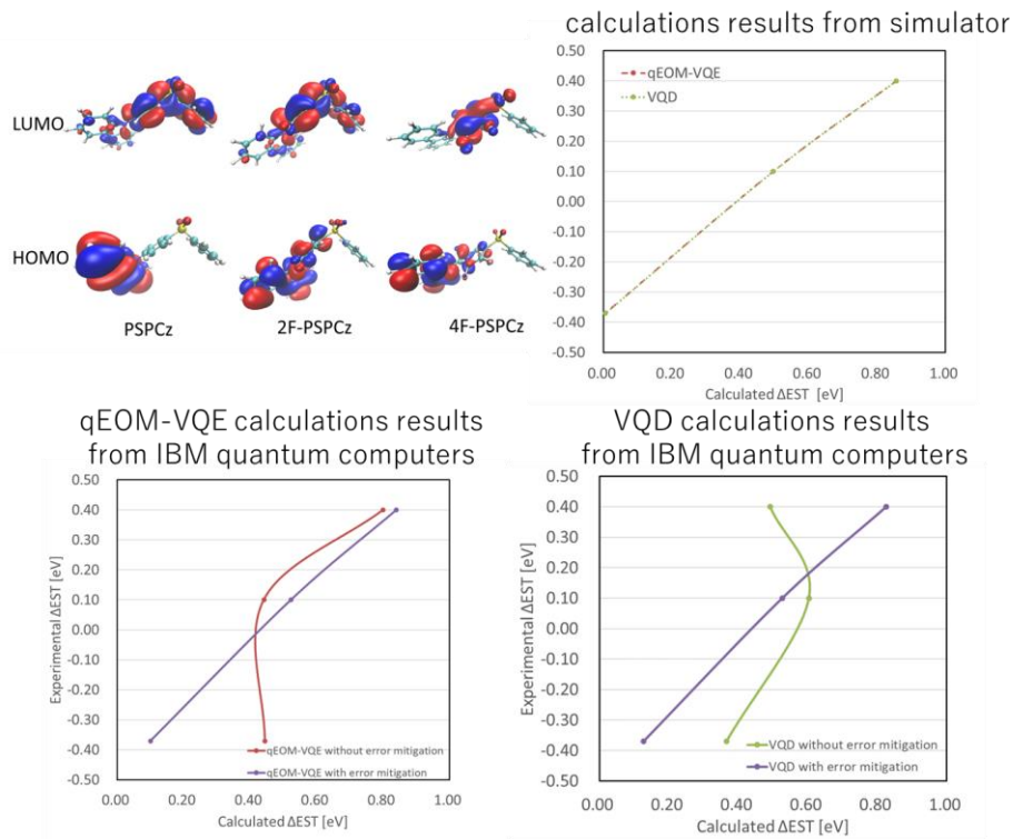
Fig. 1: Molecular structures and orbitals of TADF materials (PSPCz, 2F-PSPCz, and 4F-PSPCz) and correlations between calculation results and experiment data
